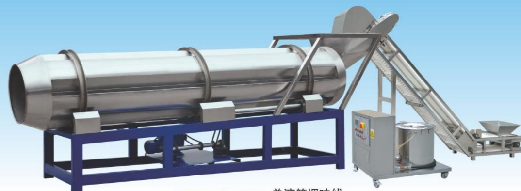
GTW-D-II 单滚筒调味线 Flavoring Line
